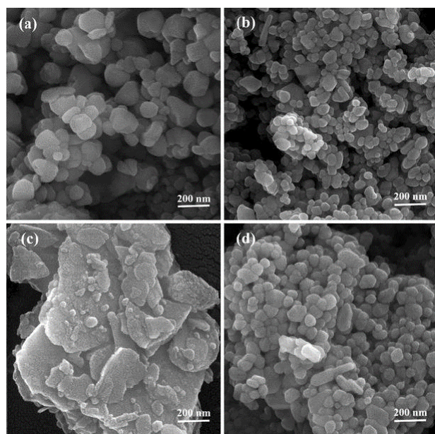
Figure 1. FE-SEM images: (a) Fe_3O_4@Alg-ZnO nanocomposite (1:10), (b) Fe_3O_4@Alg-ZnO nanocomposite (1:20), (c) Fe_3O_4 and (d) ZnO nanocrystallite
