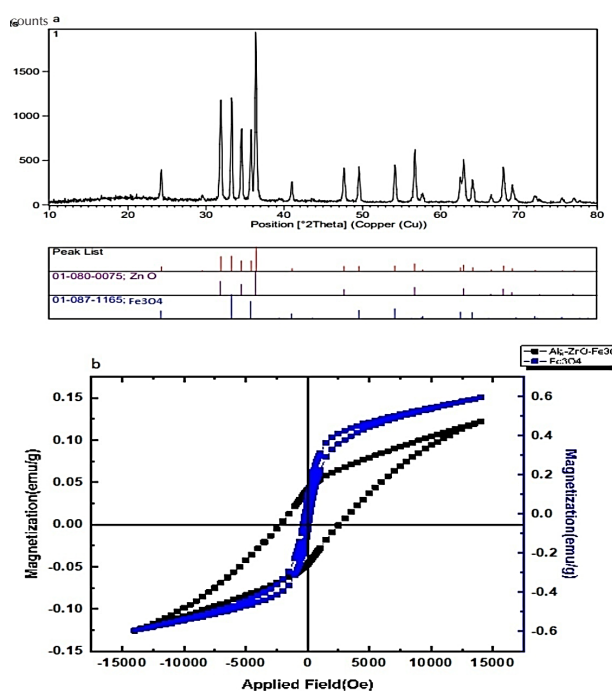
Figure 2. Characterization of Fe_3O_4@Alg-ZnO nanocomposite: (a) XRD and (b) VSM
