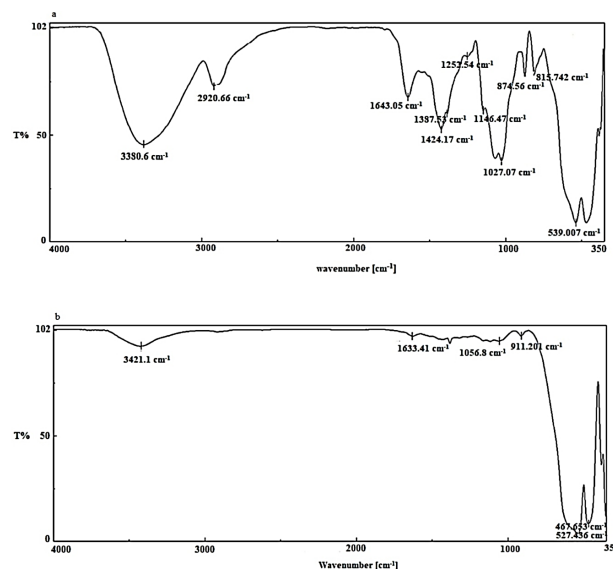
Figure 3. FTIR spectra of (a) the Fe_3O_4@Alg-ZnO nanocomposite and (b) Fe_3O_4 nanoparticles
